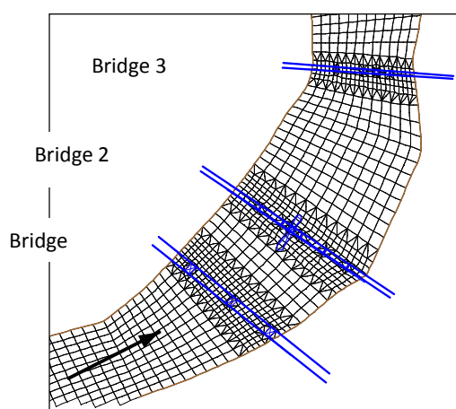
Fig. 3. Mesh generation
